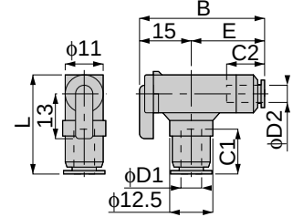
Different Diam. Union Elbow
