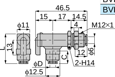
Bulkhead Union Elbow
