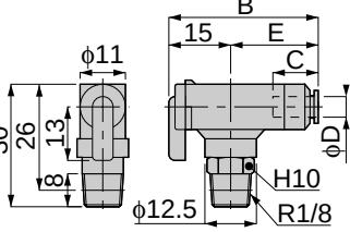
Elbow
