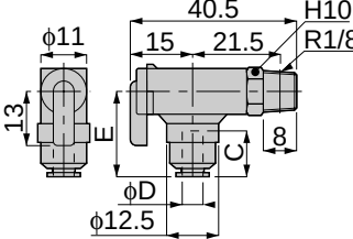
Elbow
