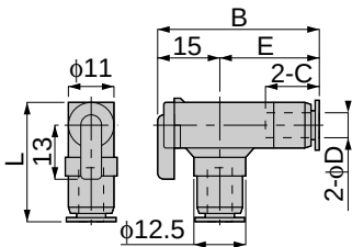
Union Elbow
