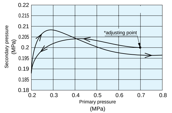
Pressure characteristics
