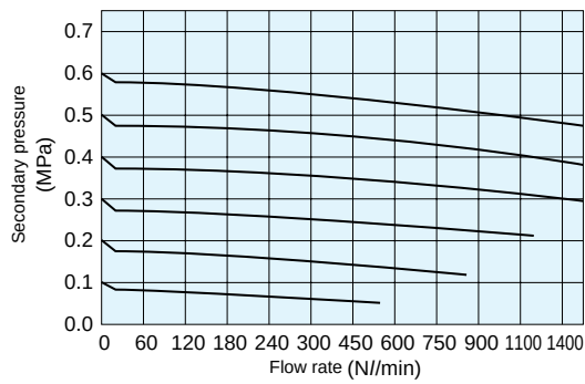
Flow characteristics
